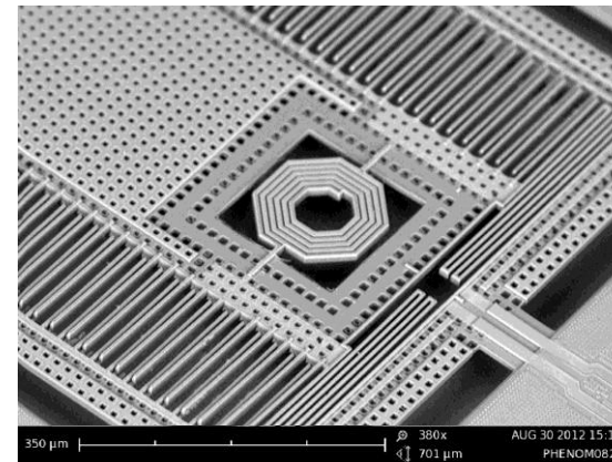
Capacitive Accelerometer
