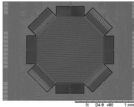
Inductive Accelerometer
