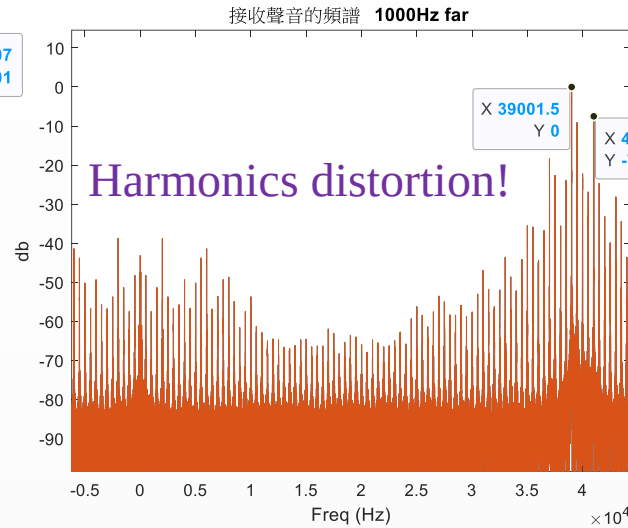
Conventional PWM
